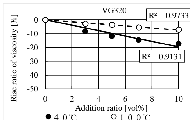
Fig.6 Rise Ratio of Viscosity for Additive Ratio
