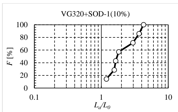
Fig.5 Weibull Diagram of VG320
