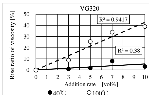
Fig.2 Rise Ratio of Viscosity for Additive Ratio
